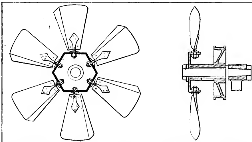
Type of fan, which permits alteration of pitch to maintain the water at an even temperature despite the variations of atmospheric conditions
